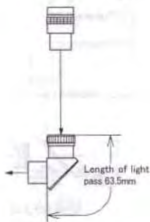
31.7(1 1/4") Prism Diagonal
