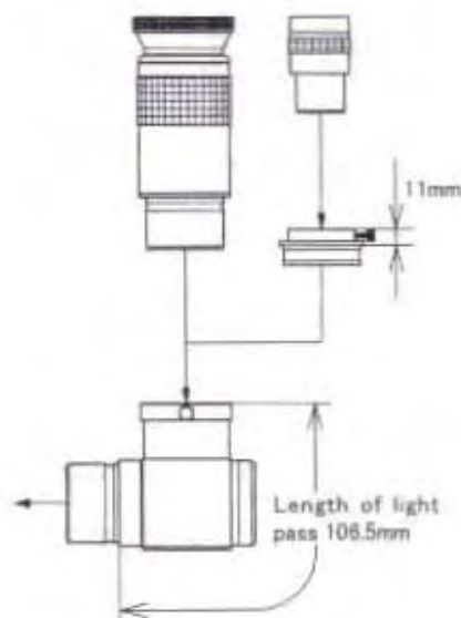
50.8(2") Mirror Diagonal
